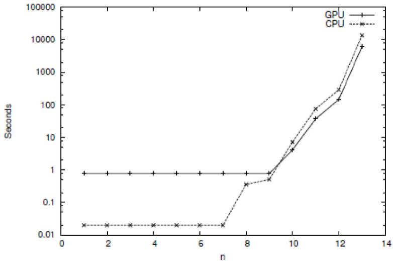
GPU vs. CPU Minimum Domination of Queen's Graph
